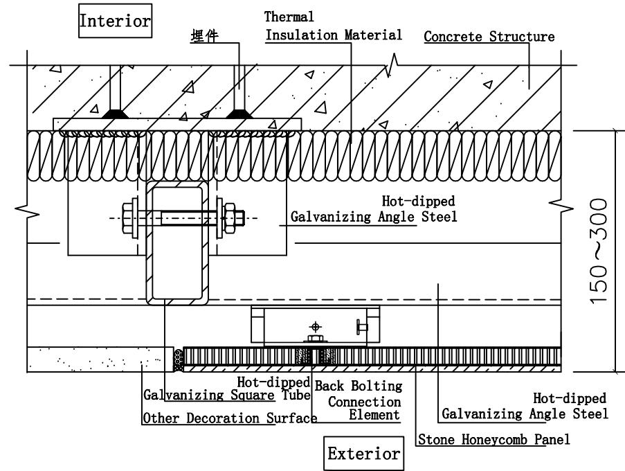
②1 Connect With Other Curtain Wall
