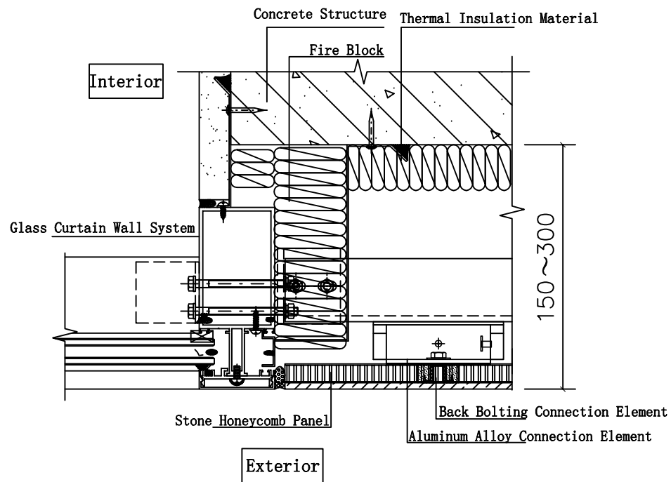
②0 Fire Block Joint
